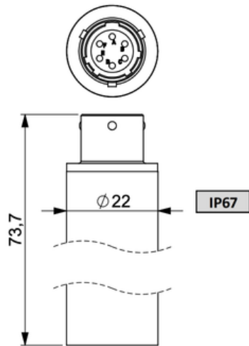
MIL-C-26482
