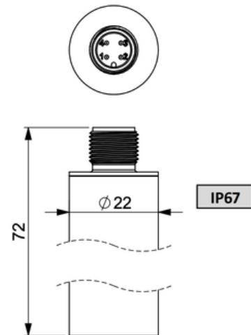
M12x1 (S763)
