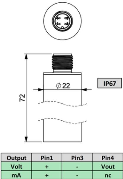
M12x1 (S763)
